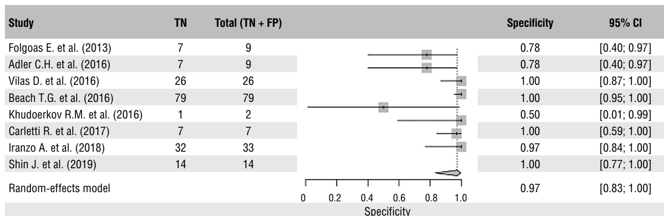
Fig. 3. Pooled sensitivity (A) and specificity (B) across the comparative studies for methods of detecting \alpha -syn in SGs of PD patients and controls using anti-pS129- \alpha -syn Abs.
